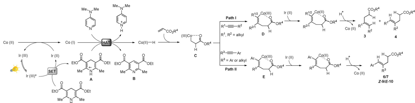
Scheme 3. Proposed mechanism for the visible-light-driven intermolecular reductive ene-yne coupling by cobalt/iridium dual catalysis.
