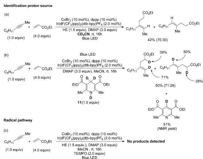
Scheme 2. Mechanistic studies.
