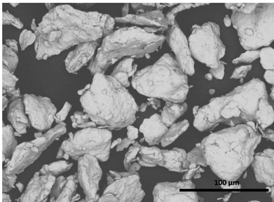
Fig. 2. Spheroidal-irregular morphology chromium used in the experiments.
