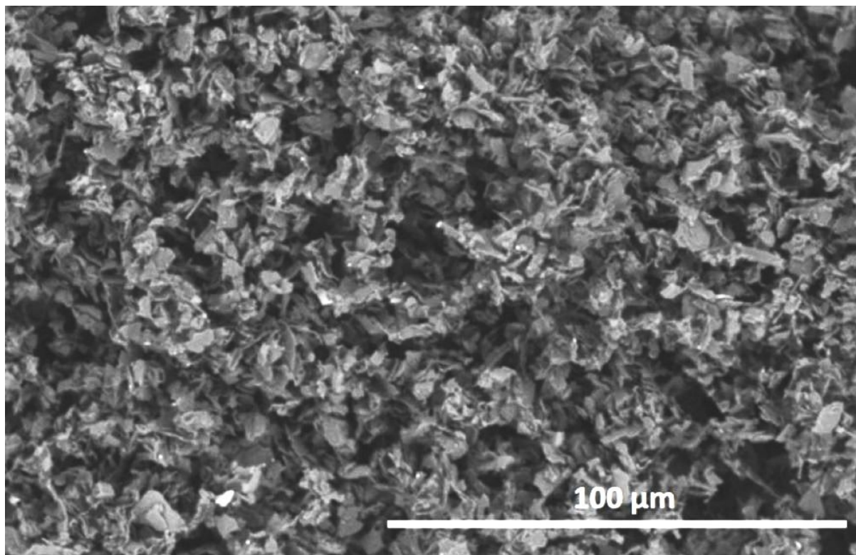
Fig. 1. Spheroidal-flake morphology graphite used in the experiments.
