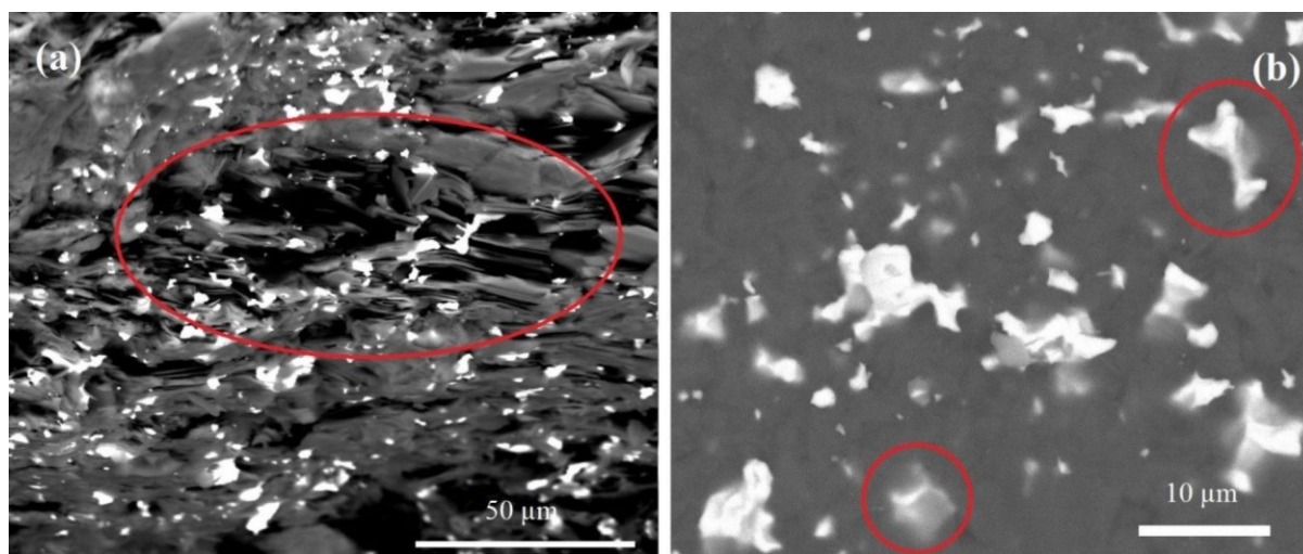
Fig. 5. SEM images of the sample graphite-7 vol. % Cr previously uniaxially pressed at 60 MPa and then SPS sintered at 1800 °C-20 min: (a) graphite lamellae oriented perpendicular to the pressing visible on fracture surface; (b) chromium carbides appear filling the spaces between grains.
