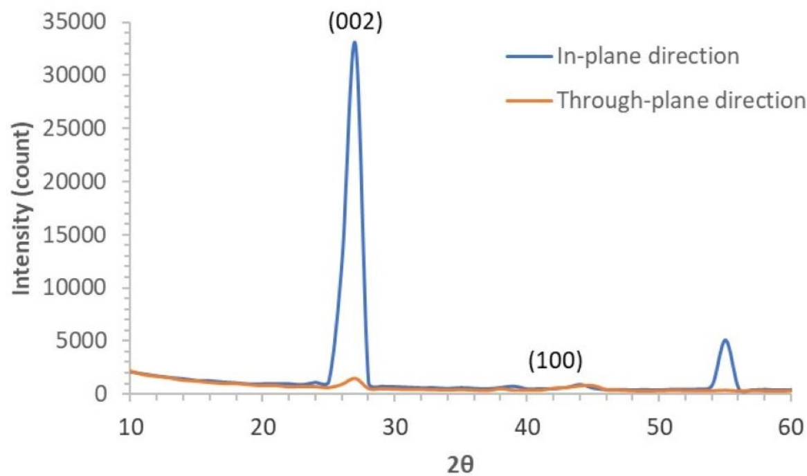
Fig. 6. X-ray diffractometer spectra of the sintered specimen graphite-7 vol. % Cr in the in-plane (blue) and through-plane (orange) directions.
