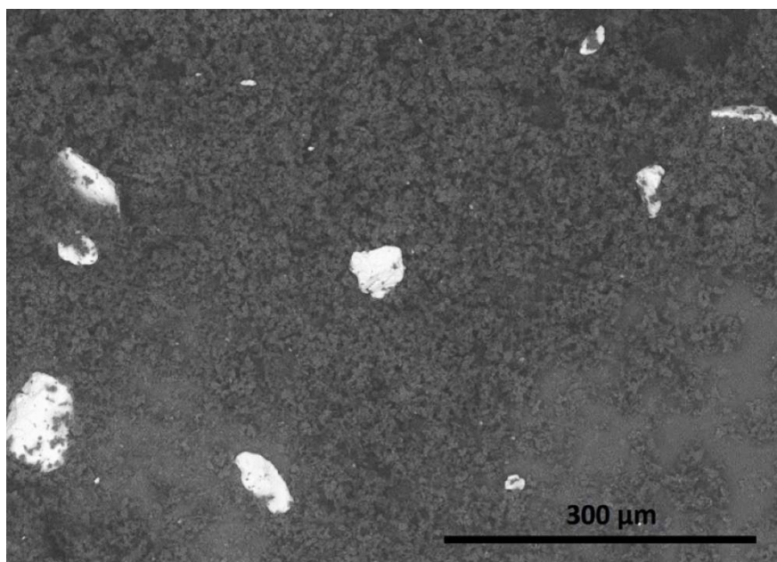
Fig. 3. Micrograph of the mixed powders, in the image, graphite-10 vol. % chromium.
