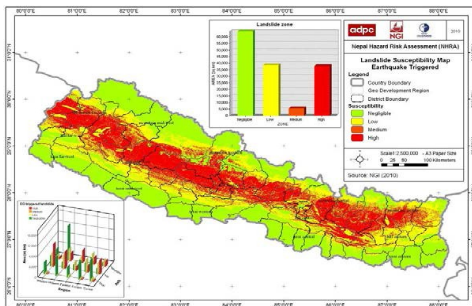
Map 3: Areas Prone to Earthquake induced landslides
