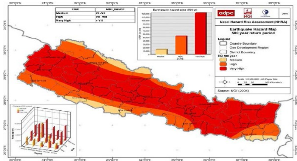
Map 3: Hazard analysis for 500 years return period
