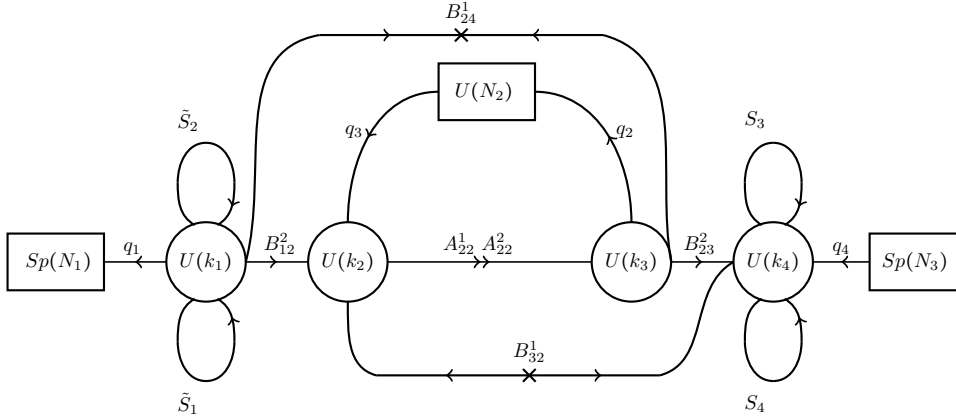
Figure 16: Quiver diagram for VS symplectic instantons on \mathbb{C}P^2/\mathbb{Z}_4 .
