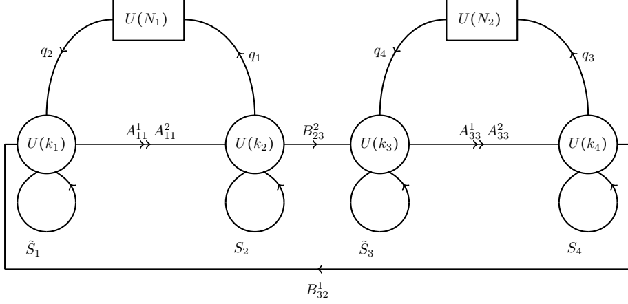
Figure 18: Quiver diagram for NVS symplectic instantons on \mathbb{C}P^2/\mathbb{Z}_4 .
