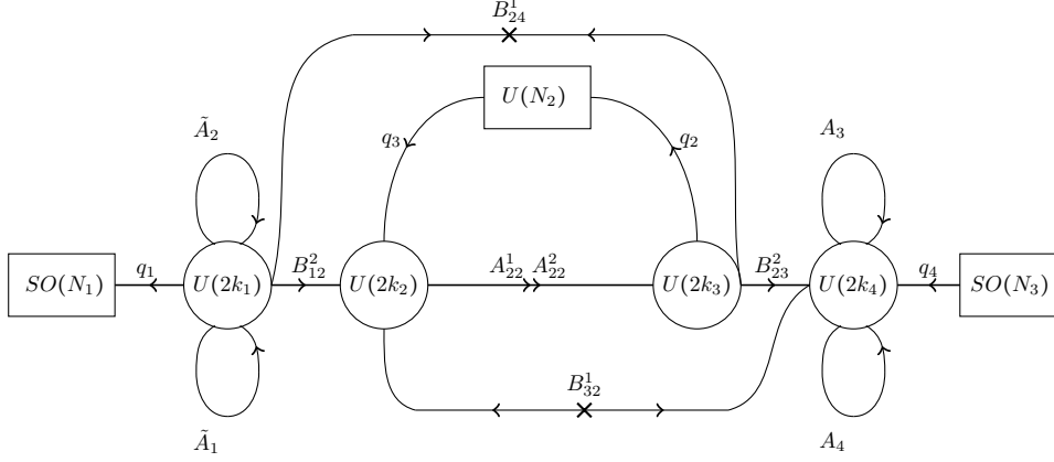
Figure 26: Quiver diagram for VS orthogonal instantons on \mathbb{C}P^2/\mathbb{Z}_4 .
