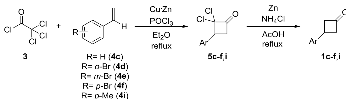
Scheme 2. General synthesis of \gamma -butyrolactones 1c-f,i .
