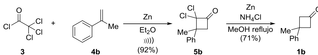
Scheme 1. Chemical synthesis of 3-phenyl-3-methylcyclobutanone ( 1b ).
