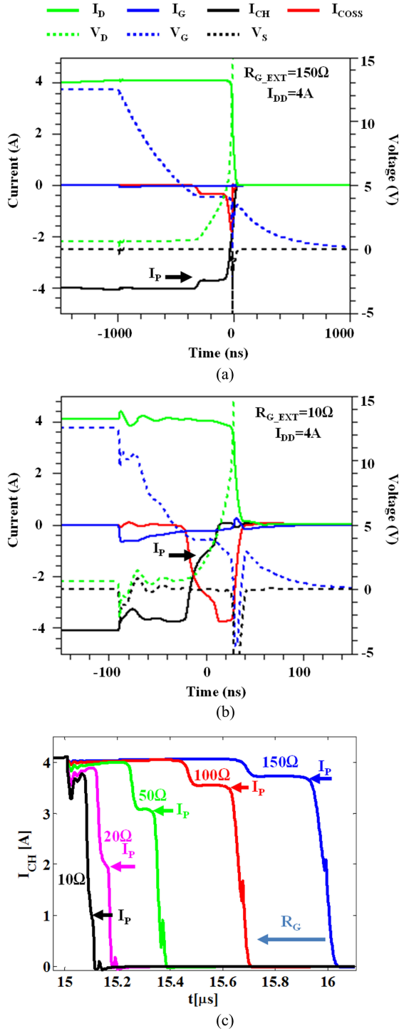
Fig. 6. Simulated current and voltage waveforms during the turn-off for (a) R_{G\_EXT} = 150\Omega and (b) R_{G\_EXT} = 10\Omega ( I_{DD} = 4A ). The I_{CH} value during the Miller plateau, otherwise named I_P , is indicated in both cases. (c) Variation of I_{CH} with R_G , in order to show the effect over the current plateau ( I_P ).
