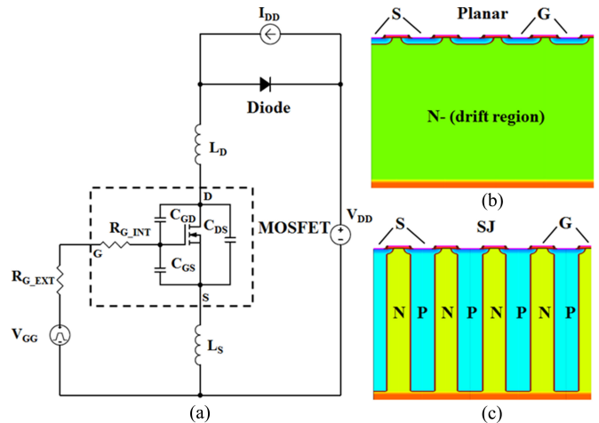
Fig. 1. (a) Circuit scheme to derive the analytical model and to perform mixed-mode simulations. (b) Cross section of Planar MOSFET. (c) Cross section of SJ MOSFET built by using TCAD tools. In the performed simulations, only a half of the basic cells in (b) or (c) are combined with the circuit in (a).
