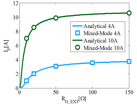
Fig. 7. I_P versus R_{G\_EXT} extracted from analytical model (lines) and simulations (symbols). I_{DD} is 4 and 10 A. I_P = I_{CH} = I_{DD} for large R_{G\_EXT} .
