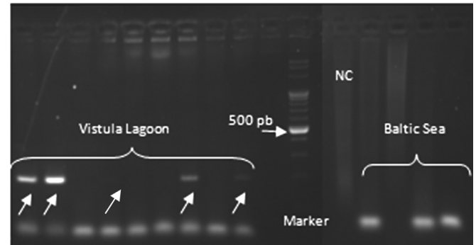
Fig. 8. Agarose gel of PCR products obtained with Rangia cuneata -specific primers in water samples from Vistula Lagoon and Baltic Sea. Positive results can be visualized with white arrows. Marker: DNA size marker 100 bp ladder. NC: negative control.
