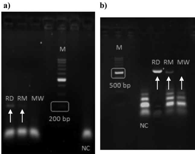
Fig. 6. a) Agarose gel of PCR products obtained with Rangia cuneata -specific primers. RD: Rangia cuneata in distilled water, RM: Rangia cuneata in marine water from Ria de Aviles (North Spain), MW: marine water from Ria de Aviles (North Spain) without Rangia cuneata . NC: negative control. M: DNA size marker 100 bp ladder. Positive results can be visualized with white arrows. b) Agarose gel of PCR products obtained with universal Palumbi primers (1996). RD: Rangia cuneata in distilled water, RM: Rangia cuneata in marine water from Ria de Aviles (North Spain), MW: marine water from Ria de Aviles (North Spain) without Rangia cuneata . NC: negative control. M: DNA size marker 100 bp ladder. Positive results can be visualized with white arrows.
