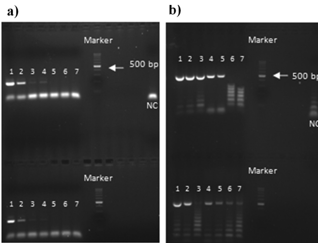
Fig. 7. a) Agarose gel of PCR products obtained with Rangia cuneata -specific primers. Upper part: Serial dilutions 1:5 to 1:15,625 of Rangia cuneata in distilled water (1–7). NC: negative control. Marker: DNA size marker 100 bp ladder. Bottom part: Serial dilutions 1:5 to 1:15,625 of Rangia cuneata together with 50 ng/μl of each other 5 mollusks (1–7). Marker: DNA size marker 100 bp ladder. b) Agarose gel of PCR products obtained with Universal primers (Palumbi, 1996). Upper part: Serial dilutions 1:5 to 1:1000 of Rangia cuneata in distilled water (1–7). NC: negative control. Marker: DNA size marker 100 bp ladder. Bottom part: Serial dilutions 1:5 to 1:1000 of Rangia cuneata with 50 ng/μl of each other 5 mollusks (1–7). Marker: DNA size marker 100 bp ladder.
