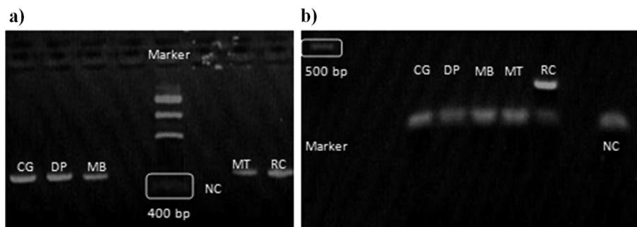
Fig. 5. a) Agarose gel of PCR products with universal primers (Palumbi, 1996) from C. glaucum (CG), D. polymorpha (DP), M. balthica (MA), M. trossulus (MT) and Rangia cuneata (RC). NC: negative control. Marker: Low DNA Mass Ladder. b) Agarose gel of PCR products with Rangia cuneata -specific primers from C. glaucum (CG), D. polymorpha (DP), M. balthica (MA), M. trossulus (MT) and Rangia cuneata (RC). NC: negative control. Marker: Low DNA Mass Ladder.
