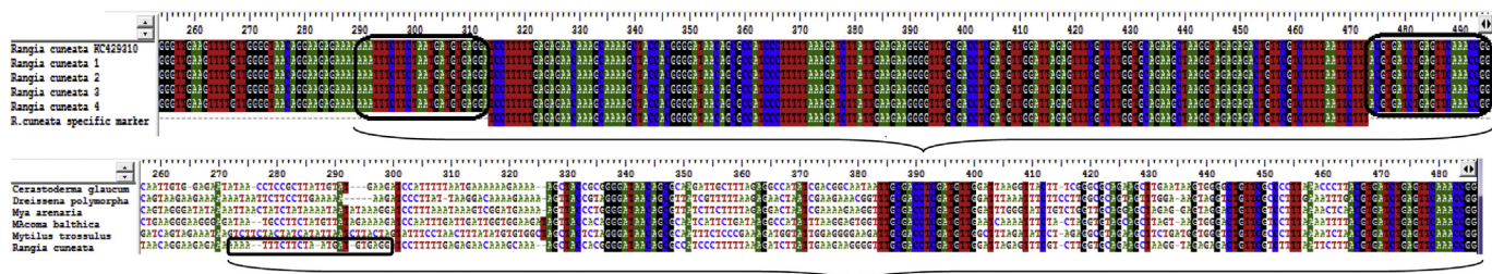
Fig. 3. Rangia cuneata -specific primer design. Alignment obtained from ClustalW tool included in BioEdit software. Upper part: alignment between different sequences of Rangia cuneata including one from GenBank (KC429310). Bottom part: alignment between 6 different mollusks species: Cerastoderma glaucum , Dreissena polymorpha , Mya arenaria , Macoma balthica , Mytilus trossulus and Rangia cuneata .
