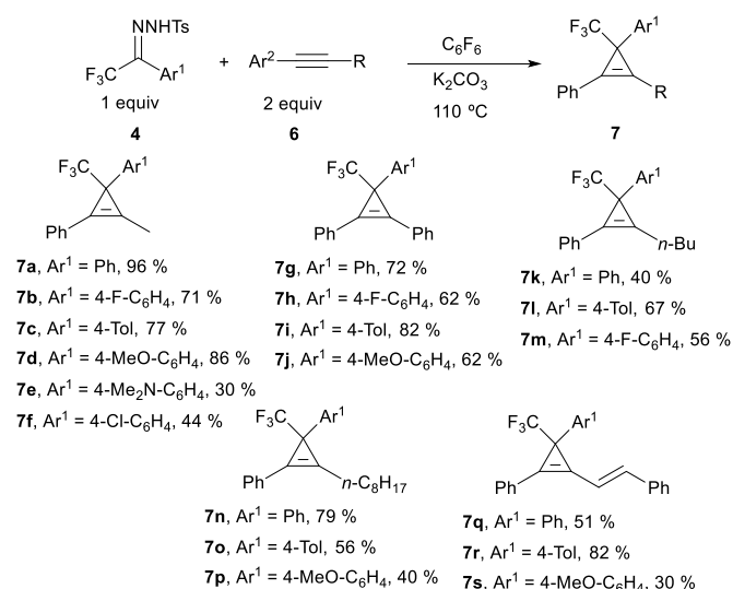
Scheme 3: Synthesis of 2-substituted-1,3-diaryl-3-trifluoromethylcyclopropenes 7 by reaction of tosylhydrazones 4 with internal alkynes.
