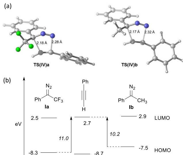
Figure 2: Figure 2. (a) Transition structures TS(IV) obtained for the 1,3-dipolar cycloadditions of phenylacetylene with the 1-(dialzo-2,2,2-trifluoroethyl)benzene Ia and 1-dialzoethylbenzene Ib respectively obtained at the M06-2X/6-311++G** level. (b) Representation of the energies of the Frontier Orbitals responsible for the main interactions in the 1,3-dipolar cycloaddition. Frontier Orbital Energies (eV) have been obtained from a single point HF/6-311G** calculation on the geometries optimized at the M06-2X/6-311++G** level.
