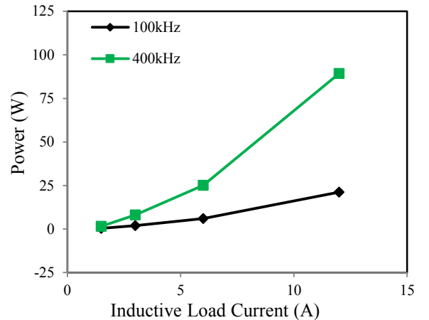
Fig. 12. Power saved when the same SJ-FET is used in CC instead of standalone configuration for different switching frequencies versus current.
