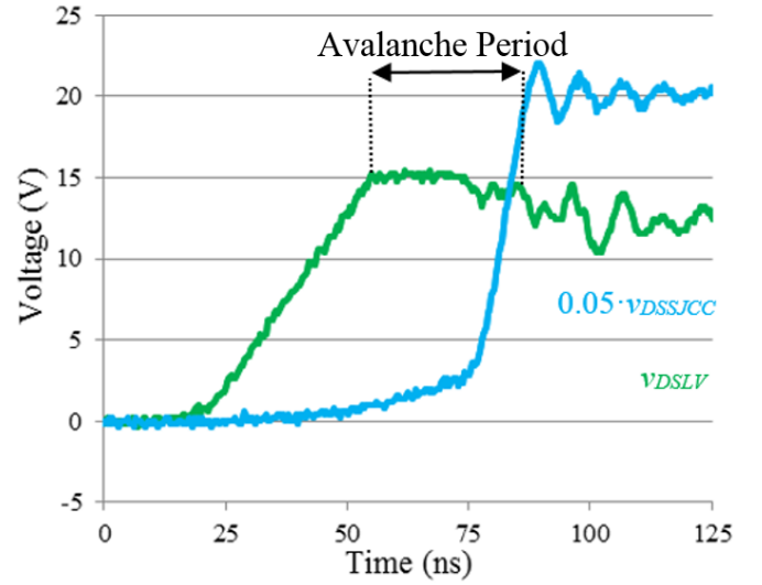
Fig. 5. Experimental waveforms of the drain to source voltage of the LV-FET and the total drain to source voltage of the SJ-CC (scaled) during the avalanche state of the LV-FET.
