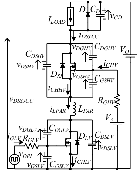
Fig. 3. Schematic circuit used to study the switching behaviour of the SJ-CC, which includes the most important parasitic elements.
