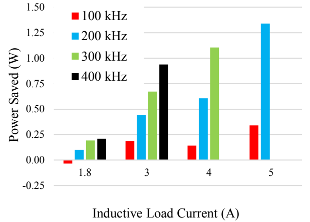
Fig. 13. Power saved when the same SJ-FET is used in CC instead of standalone configuration when the switching frequency and the current through the inductive load are modified.
