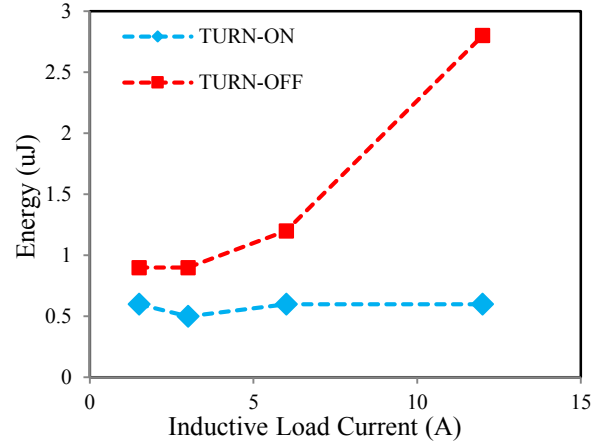
Fig. 11. Comparison of the energy dissipated by the LV-FET during both transitions.
