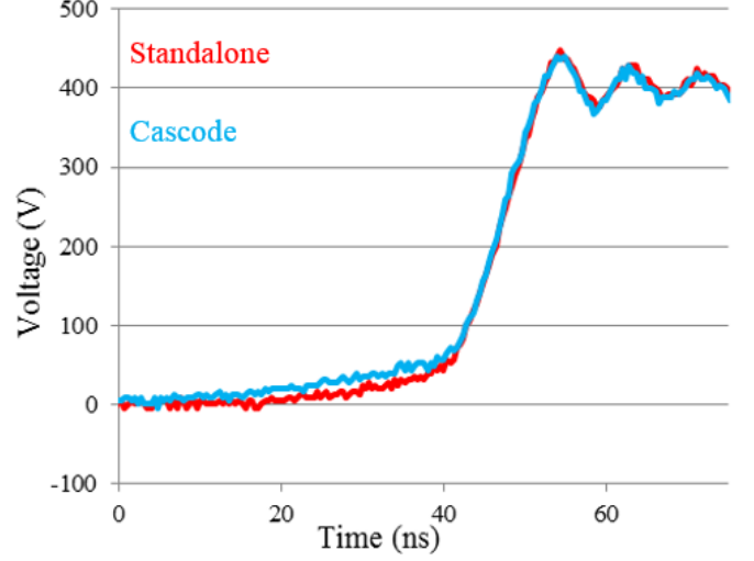
Fig. 7. Comparison between the experimental waveforms of the drain to source voltage during the turn-off of the same SJ-FET in CC and in standalone configuration.
