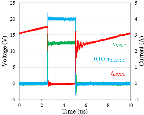
Fig. 2. Main waveforms of the boost converter at 100 kHz and 300W (100 V to 400 V).
