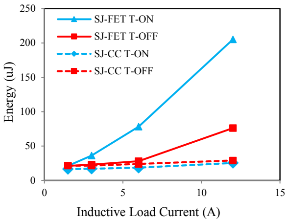
Fig. 10. Comparison of the energy dissipated by the same SJ-FET during both transitions when it is used in CC and in standalone configuration.
