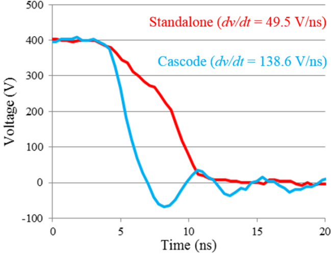
Fig. 6. Comparison between the experimental waveforms of the drain to source voltage during the turn-on of the same SJ-FET in CC and in standalone configuration.
