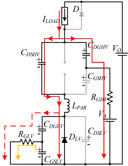
Fig. 4. Equivalent circuit of the model shown in Fig. 3 during the avalanche state of the LV-FET. The current paths provided by the inductive load ( I_{LOAD} ) are highlighted in red.
