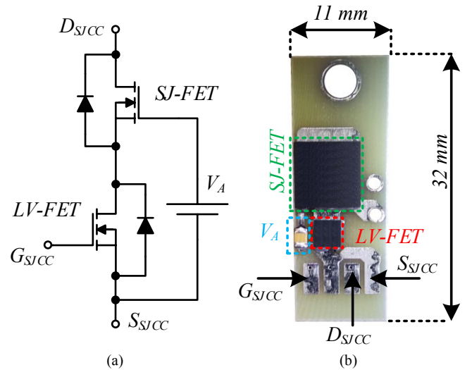
Fig. 1. SuperJunction Cascode Configuration (SJ-CC): (a) Ideal circuit schematic. (b) Plug-in board with SJ-CC prototype.
